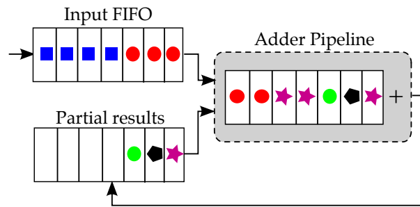
Figure 4.1: Reduction Circuit
