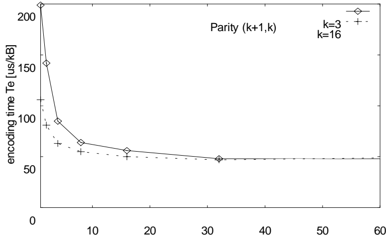
Figure 6: Encoding time T_e vs. symbol size s .
