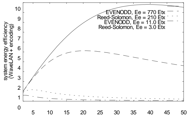
Figure 19: Energy efficiency of error correction on systems with WaveLAN.
