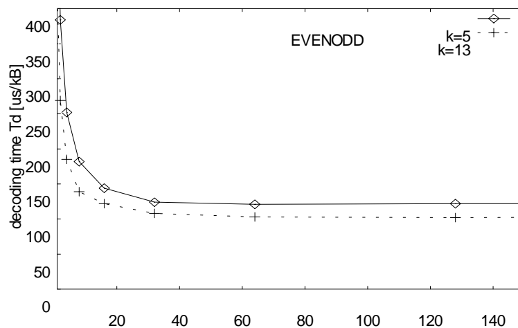
Figure 10: Decoding time T_d vs. symbol size s .
