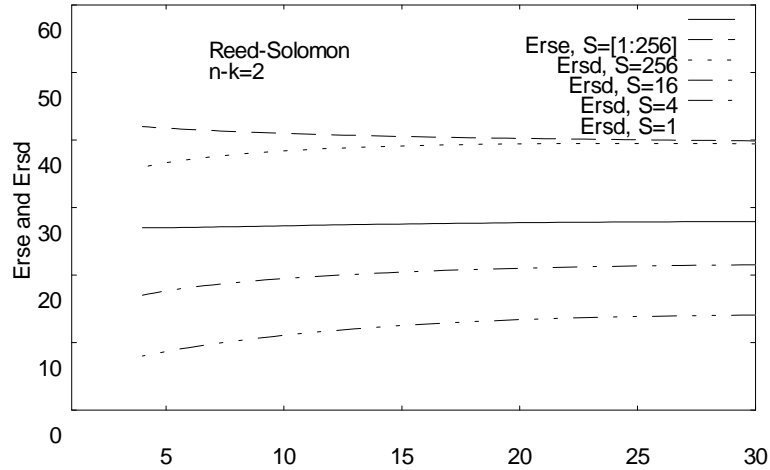
Figure 17: Energy efficiency factor vs. number of source packets for various packet sizes (in ATM cells).
