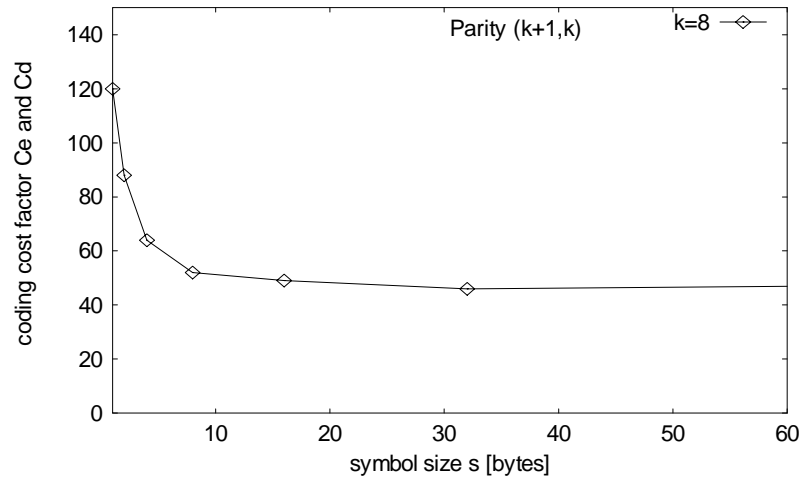
Figure 7: Encoding factor C_e vs. symbol size s .
