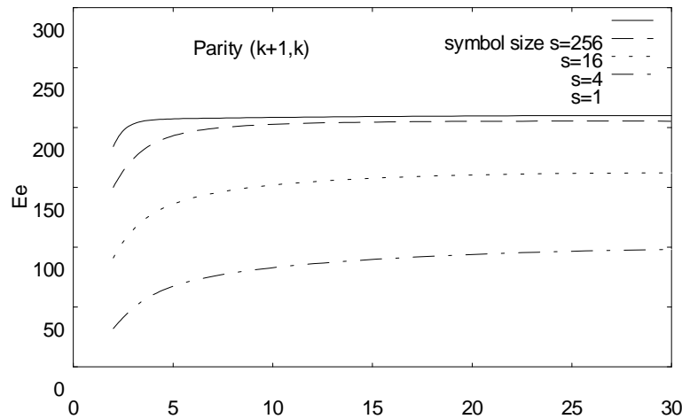
Figure 8: Energy efficiency factor E_e vs. the number of source packets k for various symbol sizes.
