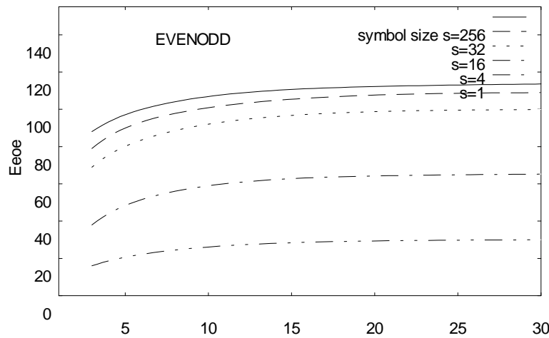
Figure 12: Energy efficiency factor E_{eoe} vs. the number of source packets k for various symbol sizes (in bytes).
