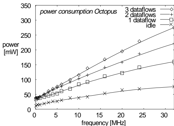
Figure 7: Power consumption Octopus switch.
