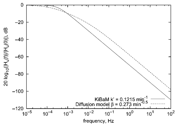
Figure 9 Frequency response for KiBaM and diffusion model
