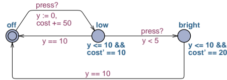
Figure 2: Model of lamp
