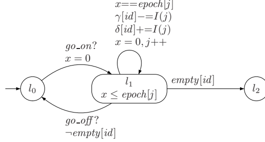
Figure 3: Discharge automaton DC
