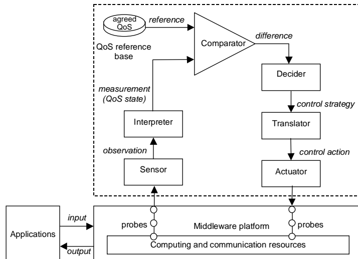
Fig. 3. QoS-control architecture.
