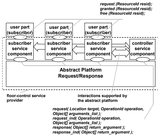
Figure 15 Structure of the callback-based floor-control service provider
