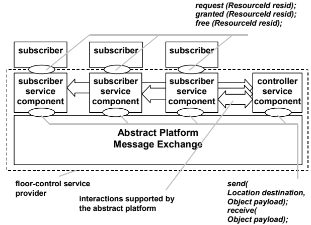
Figure 11 Structure of the callback-based floor-control service provider
