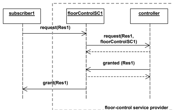
Figure 14 A resource is requested and granted (CORBA-specific realization)
