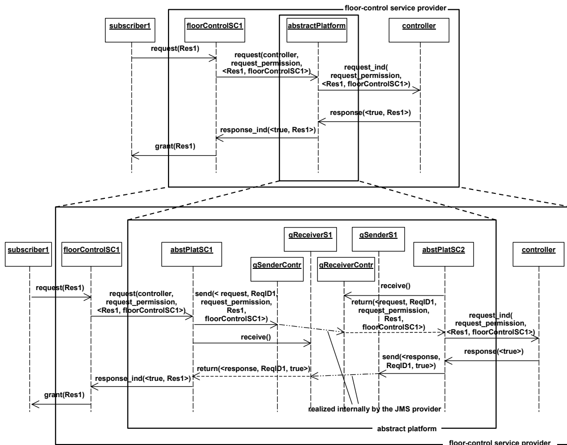
Figure 16 A resource is requested and granted
