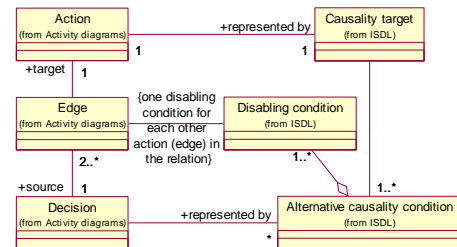
Figure 14. Mapping: UML activity diagrams - ISDL
