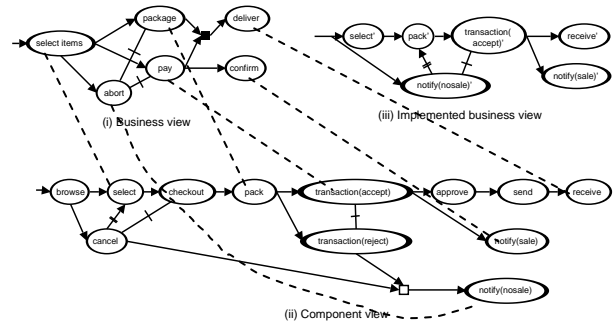
Figure 32. Refinement relation
