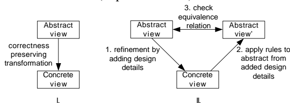
Figure 12. Refinement techniques
