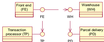
Figure 24. Application decomposition
