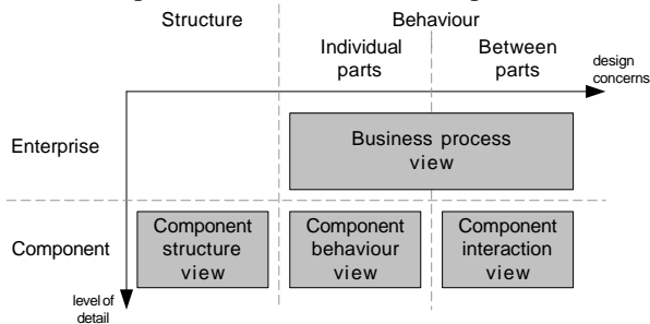
Figure 19. Application views
