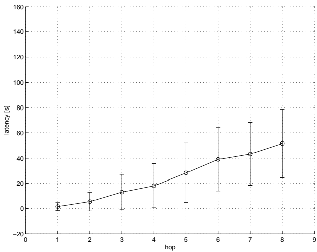
Fig. 4. Average latency and standard deviation; maximum given advice: 2 slots
