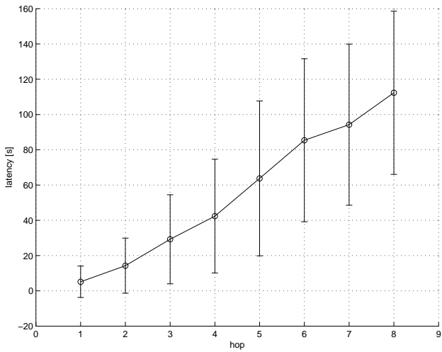
Fig. 3. Average latency and standard deviation when all nodes control one time slot
